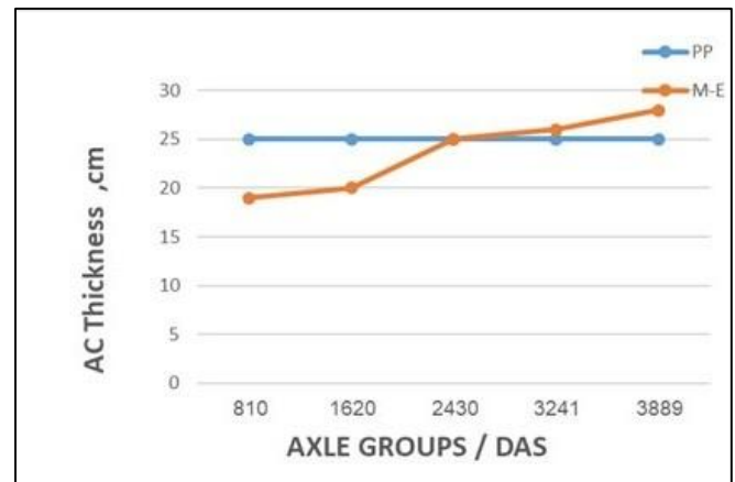
Figure 13. M-E versus Perpetual Design by axle groups
