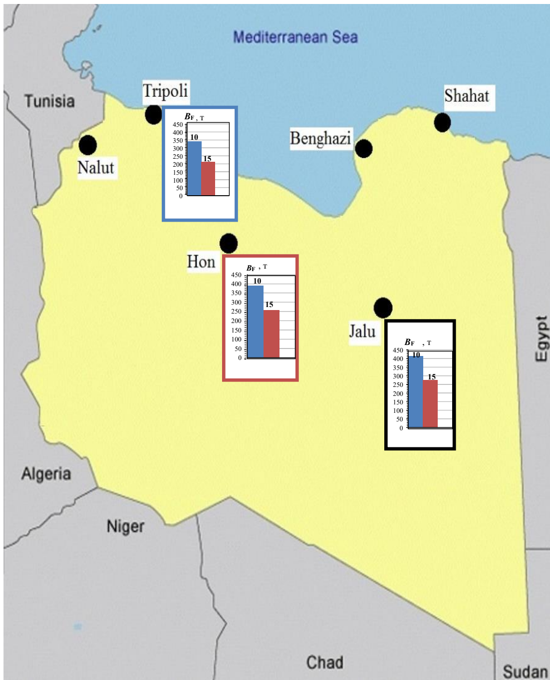
Fig.7. Values of annual fuel savings in BF due to air cooling at the gas turbine inlet from the current temperature t_a to t_{a2} = 10\text{ }^\circ\text{C} (in REC) , t_{a2} = 15\text{ }^\circ\text{C} (in ABC) , for gas turbines of power plants in 3 regions: 1 – Tripoli ; 2 - Center (Hon) ; 3 - South (Jalu).
