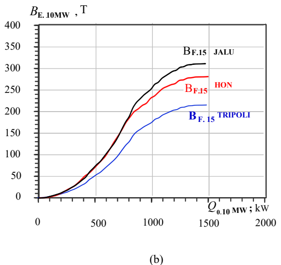
Fig.6. values of the annual specific fuel saving B_{F,10\text{MW},T} , due to cooling at the gas turbine inlet with an electric power of 10 MW depending on the corresponding costs of cooling power Q_{0,10\text{MW}} , KW, at different final temperatures of cooled air t_{a2} ( — Tripoli; — Hon; — jalu, 2009 ): B_{F,10} at t_{a2} = 10^\circ\text{C} in REC (a) and t_{a2} ( — Tripoli; — Hon; — jalu, 2009 ): B_{F,15} at t_{a2} = 15^\circ\text{C} in ABC (b).
