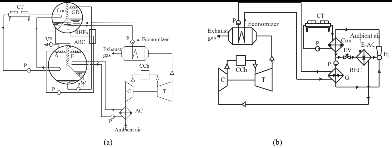
Fig. 2. Schemes of cooling systems of GT intake air in ABC (a) and REC (b) with utilization of exhaust gas heat: C – compressor; T – turbine; C C h – combustion chamber; Economizer – a water-heating utilization boiler; P – pump; ABC: GD – generator-desorber of water vapour; Con – condenser; A – absorber; E – evaporator; RHEs – regenerative heat exchanger of solutions, VP – vacuum pump; REC: E j – ejector; G – generator of refrigerant vapour; Con – condenser; E-AC – evaporator-air cooler; EV – expansion valve; CT – cooling tower.
